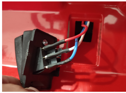
Step 1. Check the connection of pedal switch
