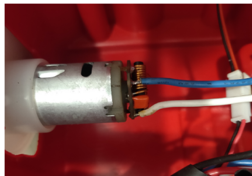
Step 5. Check the motor connection
