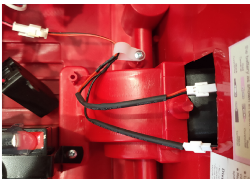
Step 4. Check the light cable connection
